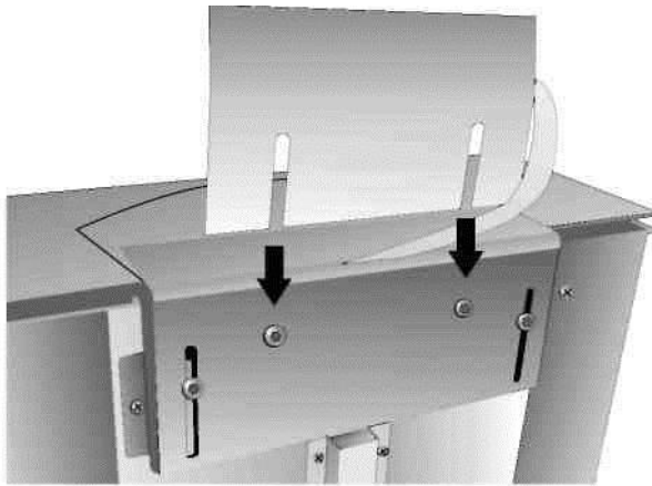
Pict. 19: passing the flat cable
