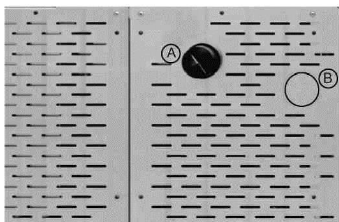
A. Horizontal air duct B. Discharge of smoke
